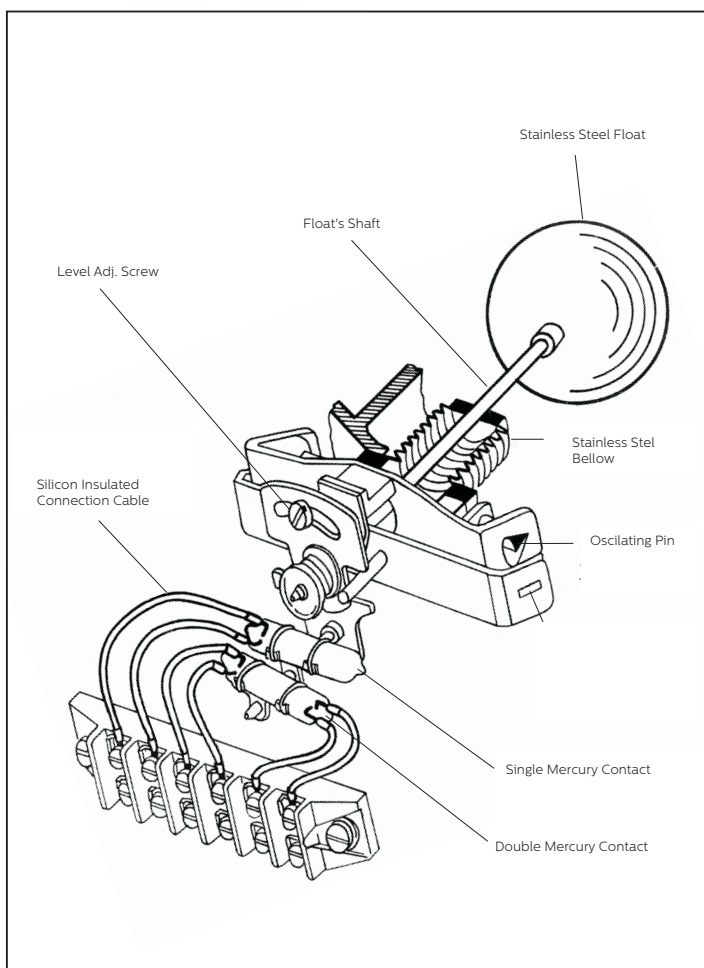
FLANGED BODY
