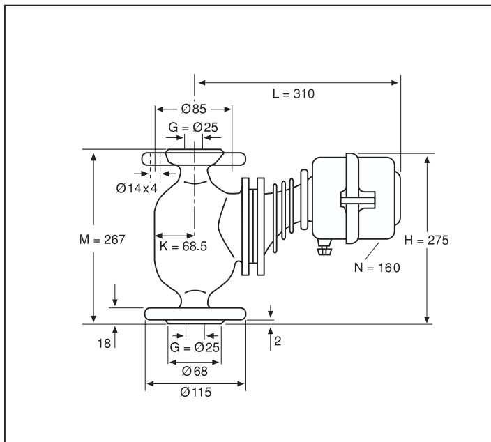
FLANGED BODY
