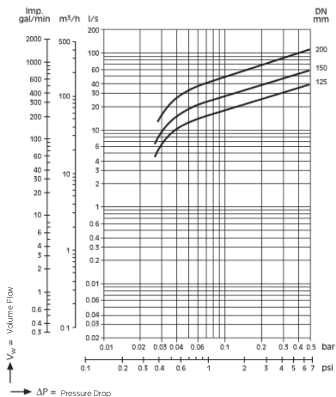
PRESSURE GRAPH
